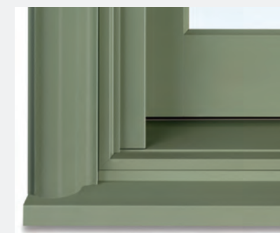
RIDGELAND CASING WITH A1453 SUBSILL
